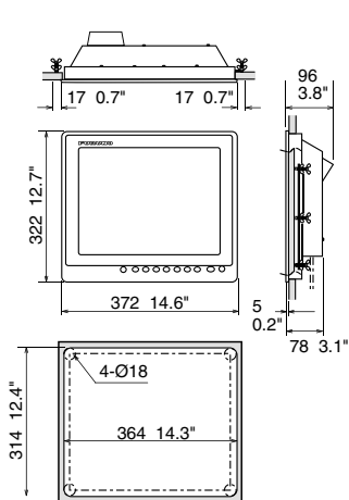
MU-150HD Flush Mount 5.4 kg 11.9 lb
