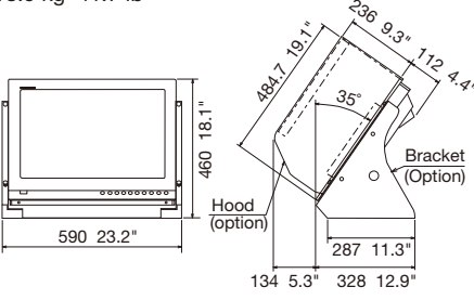
MU-231 Bracket Mount 18.9 kg 41.7 lb
