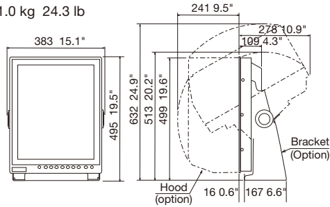
MU-190V Bracket Mount 11.0 kg 24.3 lb
