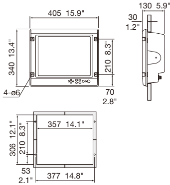
MU-151C Flush Mount 7.5 kg 17.4 lb
