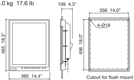
MU-190V Flush Mount 8.0 kg 17.6 lb
