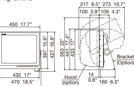
MU-190 Bracket Mount 11 kg 24.3 lb
